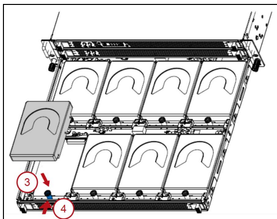
Figure 196 Install the drive.
