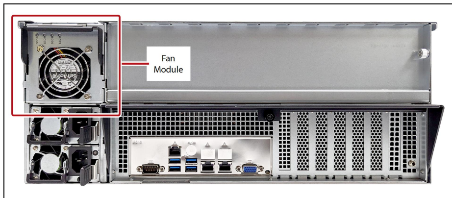
Figure 183 The NVMe drive fan module.
