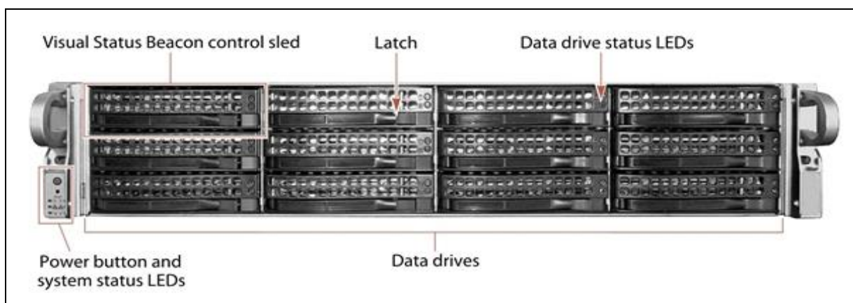
Figure 15 The front view of the Gen1 V Series BlackPearl NAS 2U master node (front bezel removed).
