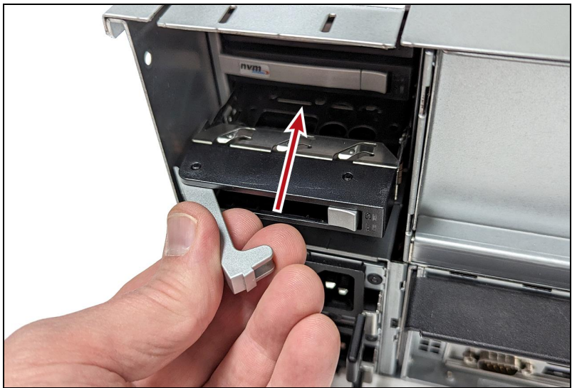
Figure 189 Insert drive into chassis.
