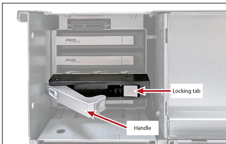
Figure 185 Unlock the drive sled.
