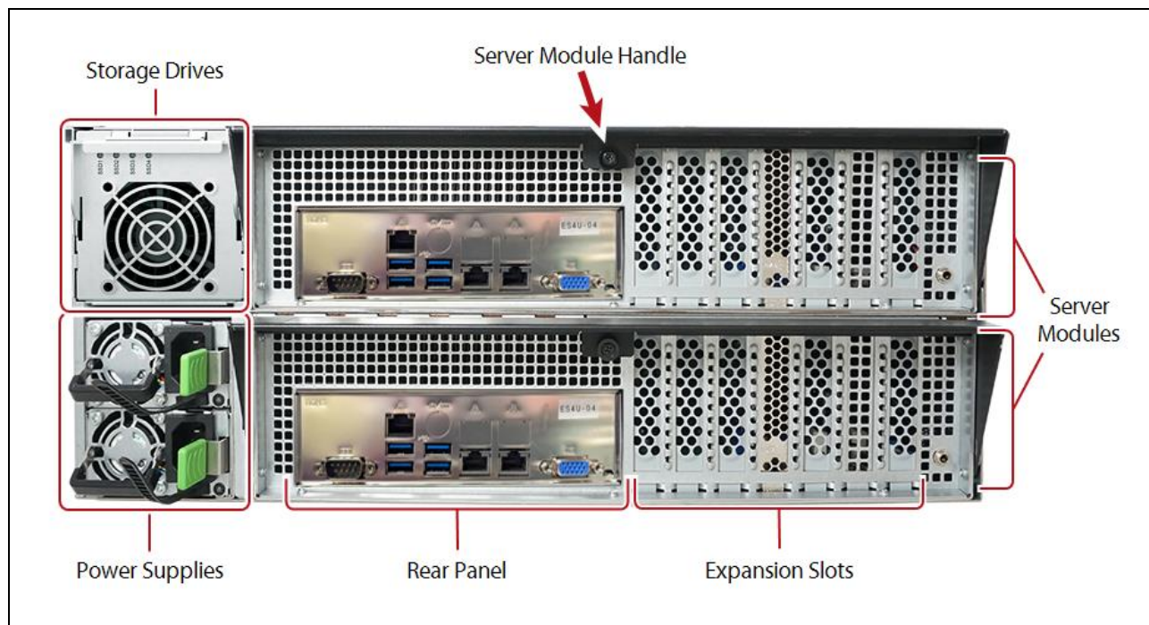
Figure 3 The rear view of the Gen3 H Series BlackPearl NAS solution.
