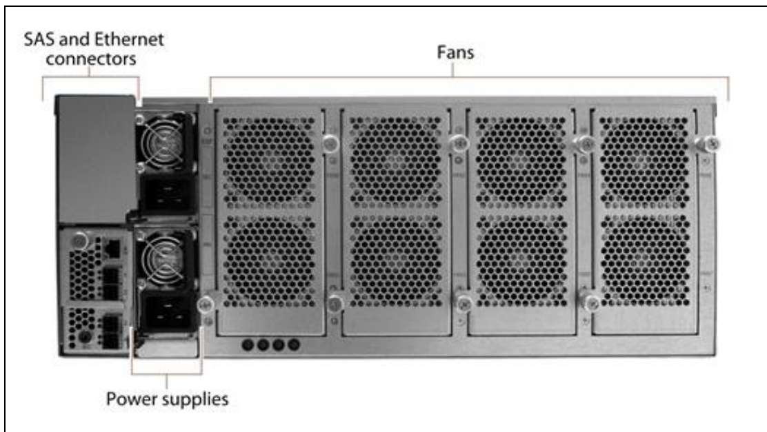
Figure 13 The rear view of the 77-bay and 107-bay expansion nodes.
