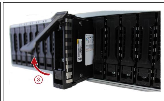
Figure 198 Remove the drive sled with drive blank and insert the drive sled with drive.
