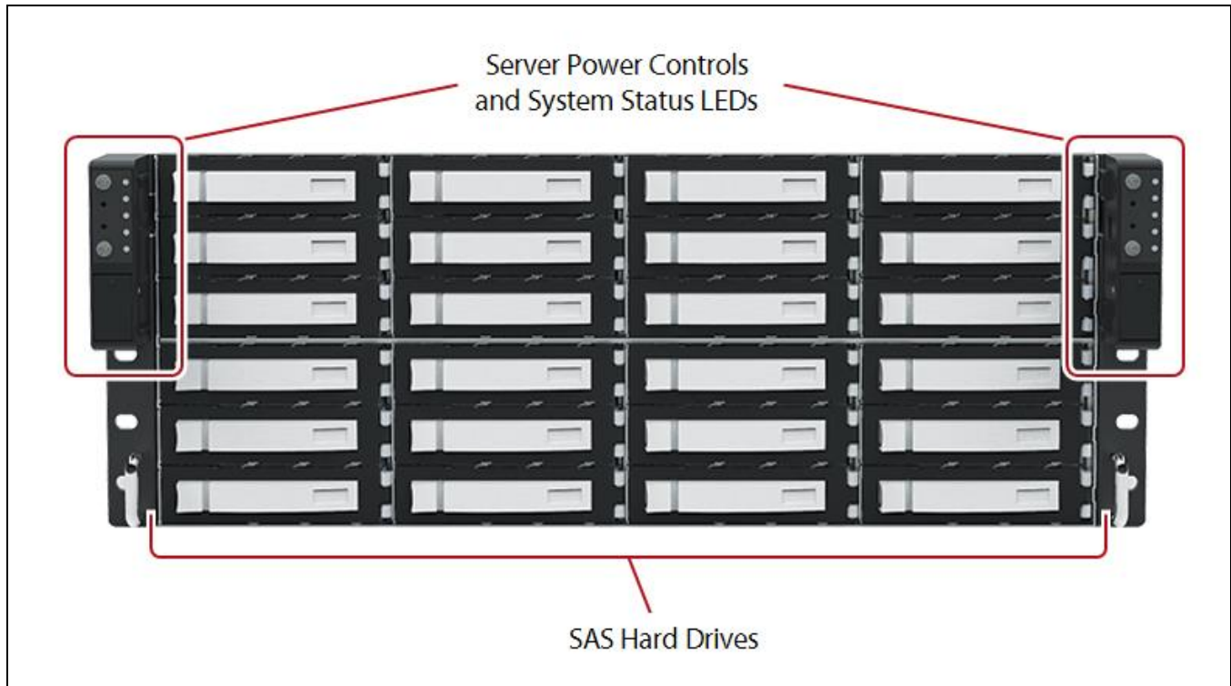
Figure 2 The front view of the Gen3 H Series BlackPearl NAS solution (front bezel removed).
