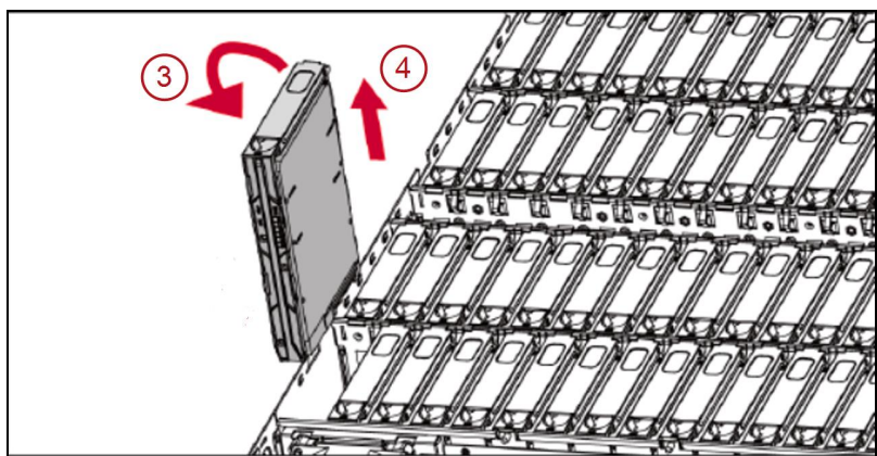
Figure 192 Remove the drive from the BlackPearl chassis.
