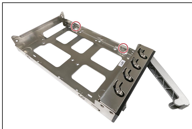
Figure 177 PEMs on right side of sled.
