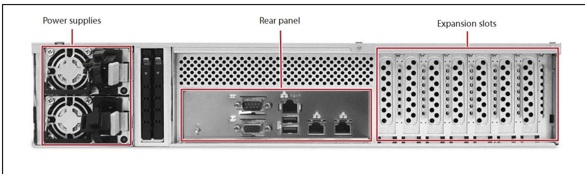
Figure 10 The rear view of the Gen2 V Series BlackPearl NAS 2U solution.
