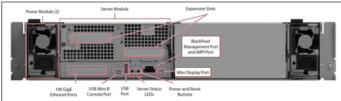
Figure 6 The rear view of the Gen2 X Series BlackPearl NAS solution.
