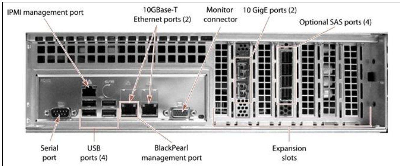
Figure 18 The Gen1 S Series BlackPearl NAS rear panel components.
