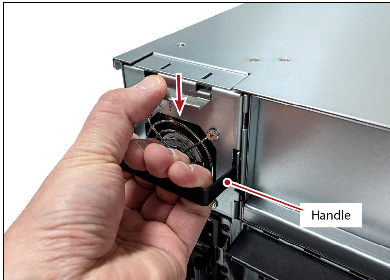
Figure 184 Remove the NVMe drive fan module.
