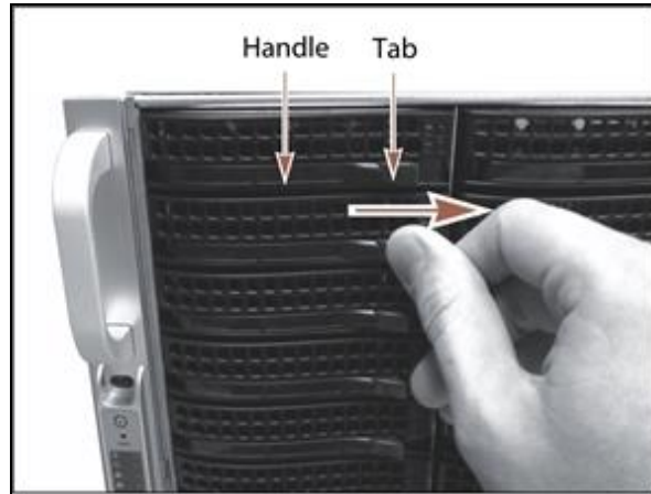
Figure 199 Slide the tab to the right to release the drive sled handle.
