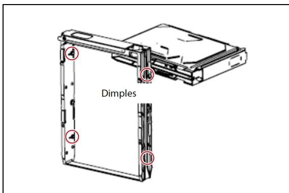
Figure 193 Match the dimples on the drive sled to the dimples on the drive.
