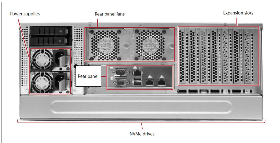
Figure 9 The rear view of the Gen2 S Series BlackPearl NAS 4U solution.
