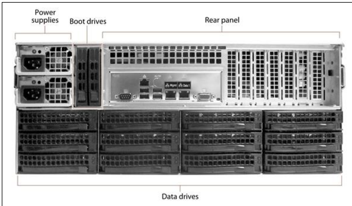
Figure 16 The rear view of the Gen1 S Series BlackPearl NAS 4U master node.
