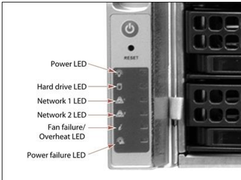
Figure 142 The left side of the front of the Gen1 S Series chassis showing system status LEDs.
