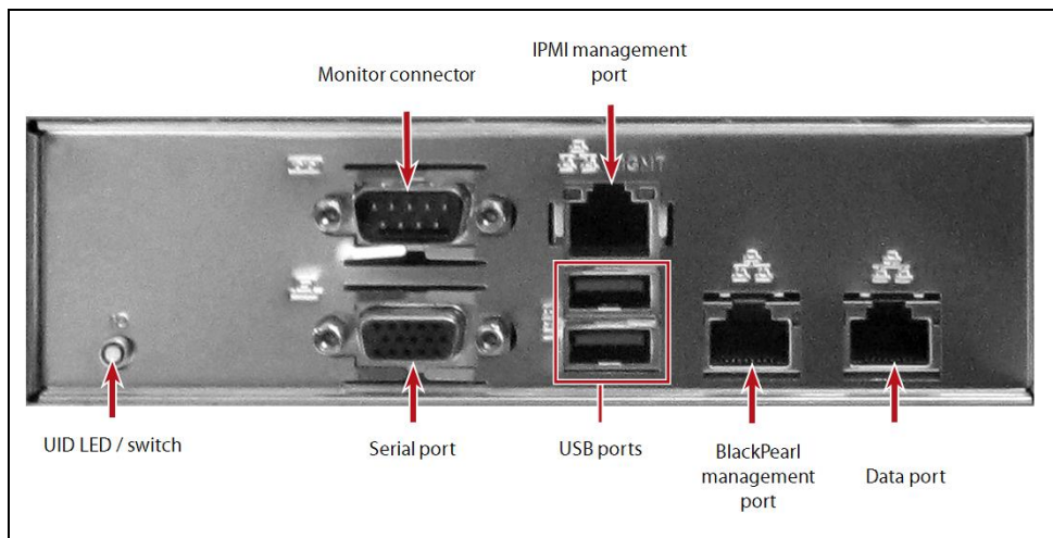
Figure 11 The Gen2 S Series and Gen 2 V Series BlackPearl NAS rear panel components.
