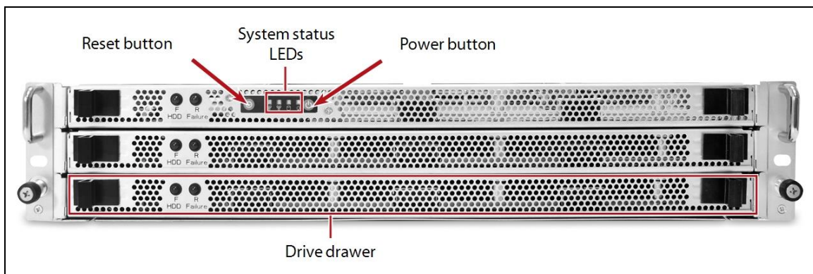
Figure 8 The front view of the Gen2 V Series BlackPearl NAS 2U solution (front bezel removed).
