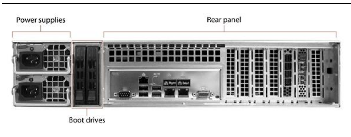
Figure 17 The rear view of the Gen1 V Series BlackPearl NAS 2U master node.
