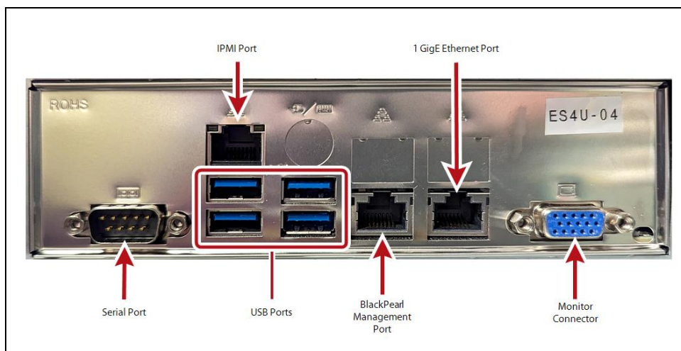
Figure 4 The Gen3 H Series BlackPearl NAS rear panel components.
