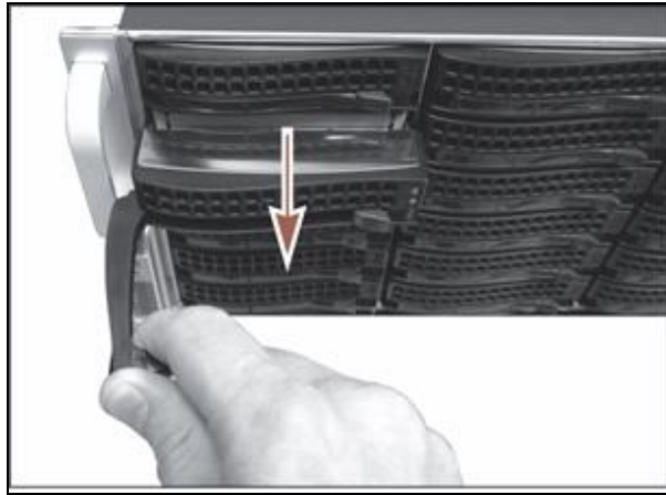
Figure 202 Pull the sled out of the solution.
