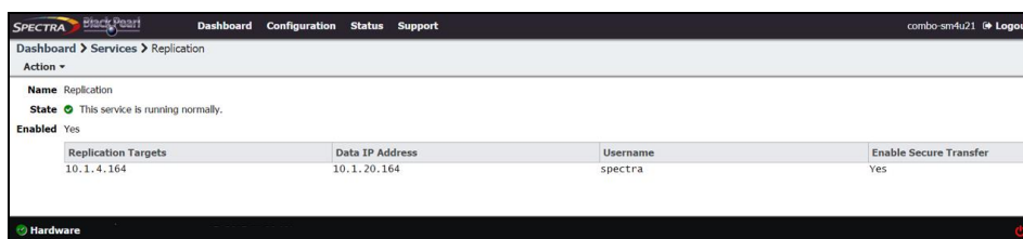
Figure 103 The Replication service details screen.
