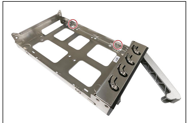
Figure 179 PEMs on right side of sled.
