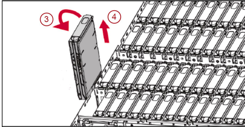
Figure 194 Remove the drive from the BlackPearl chassis.
