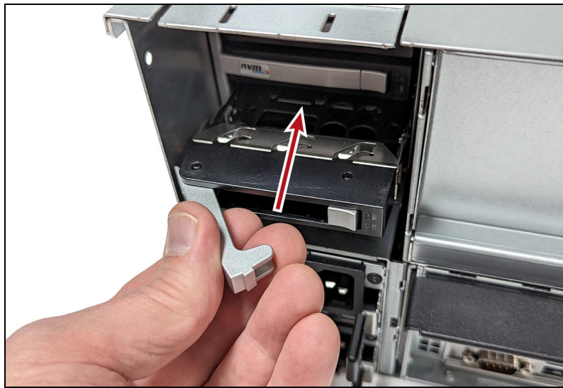
Figure 191 Insert drive into chassis.
