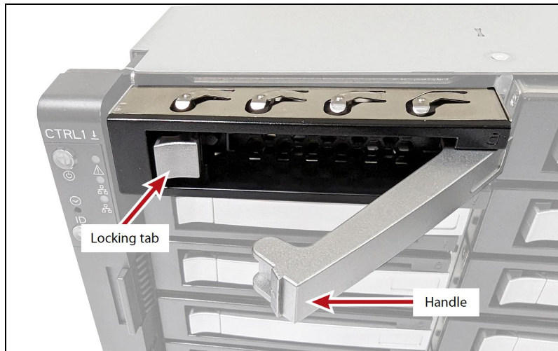
Figure 177 Unlock the drive sled.
