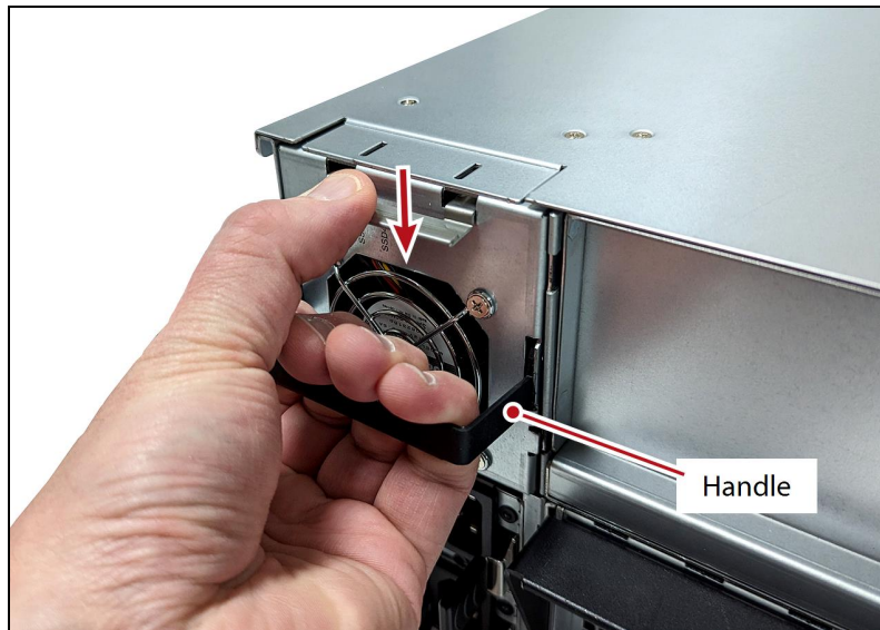
Figure 186 Remove the NVMe drive fan module.
