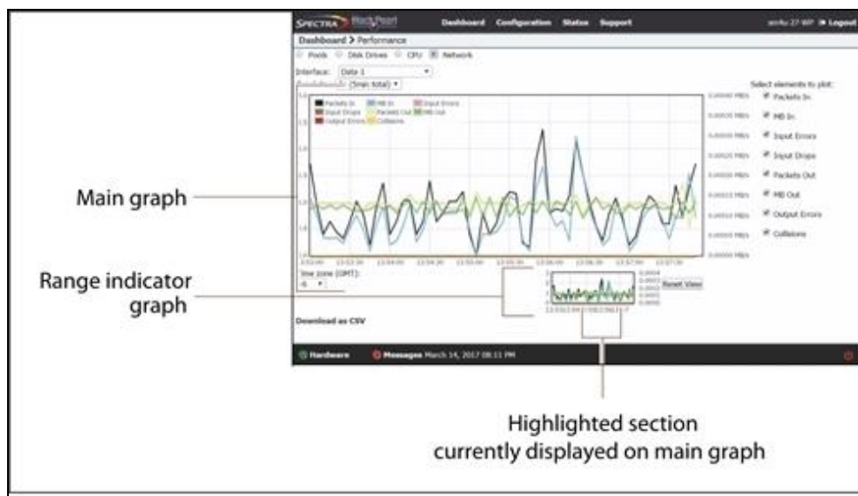
Figure 154 Highlight a section of data to show in greater detail.
