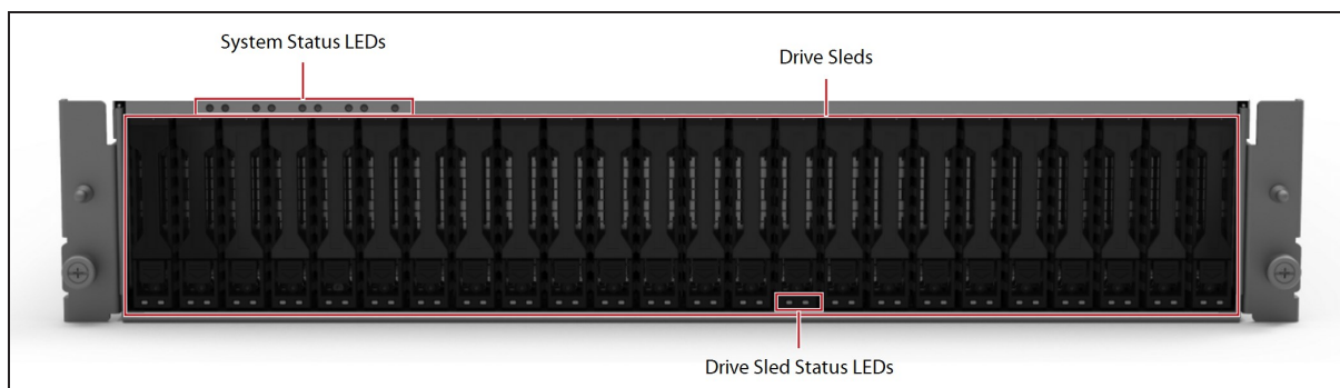
Figure 8 The front view of the Gen2 X Series BlackPearl Storage Manager (front bezel removed).
