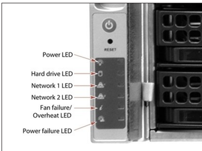
Figure 166 The left side of the front of the Gen1 S Series chassis showing system status LEDs.
