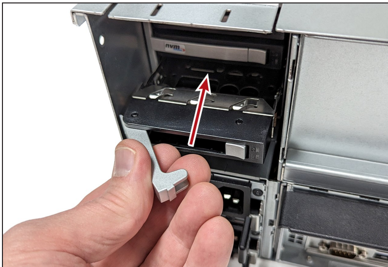
Figure 197 Insert drive into chassis.
