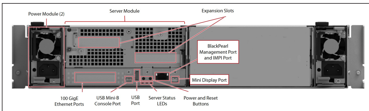
Figure 9 The rear view of the Gen2 X Series BlackPearl Storage Manager.
