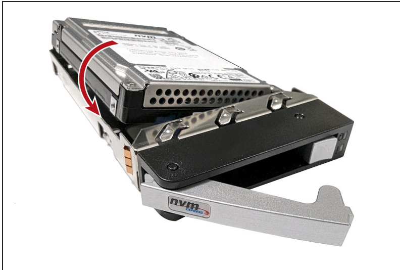
Figure 196 Install the drive into the sled.
