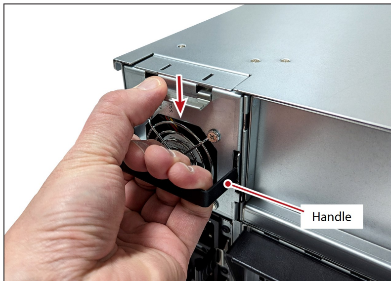
Figure 192 Remove the NVMe drive fan module.
