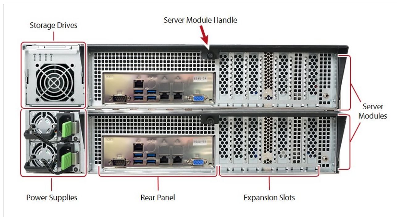
Figure 6 The rear view of the Gen3 H Series BlackPearl Storage Manager.
