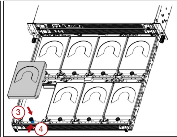
Figure 204 Install the drive.
