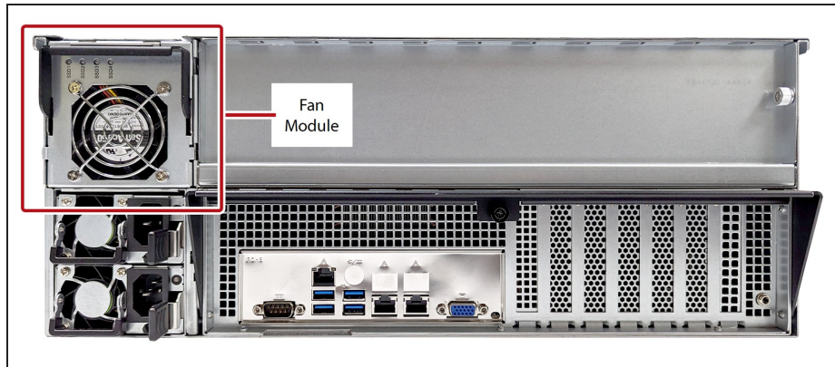
Figure 191 The NVMe drive fan module.
