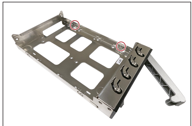
Figure 185 PEMs on right side of sled.
