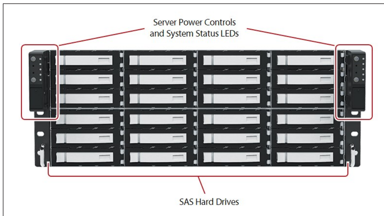
Figure 5 The front view of the Gen3 H Series BlackPearl Storage Manager (front bezel removed).
