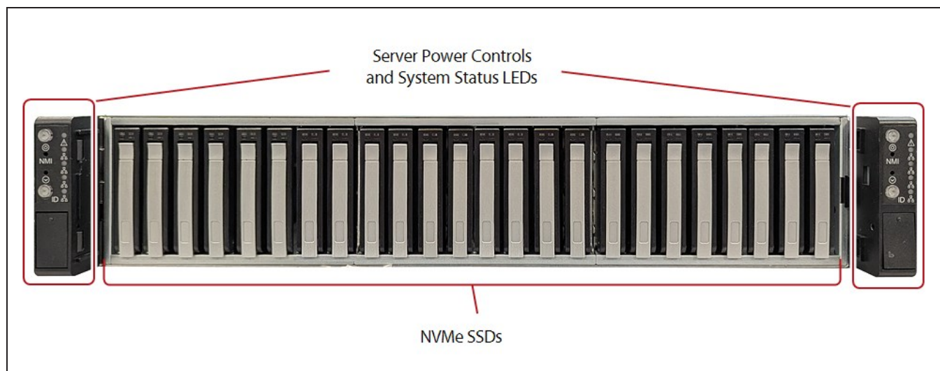
Figure 2 The front view of the Gen3 F Series BlackPearl Storage Manager (front bezel removed).
