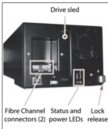
Figure 12 The TS11xx technology drive sled.
