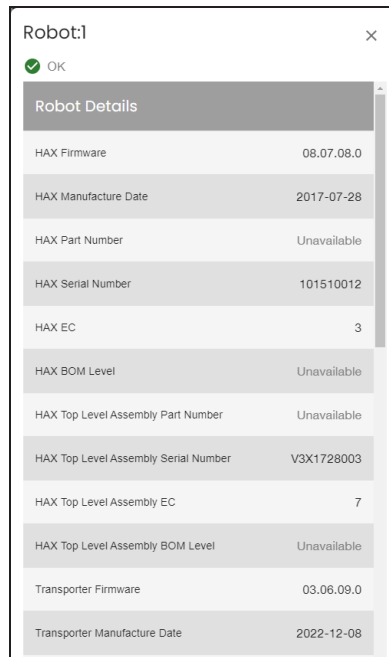
Figure 94 The LumOS Robot Details screen
