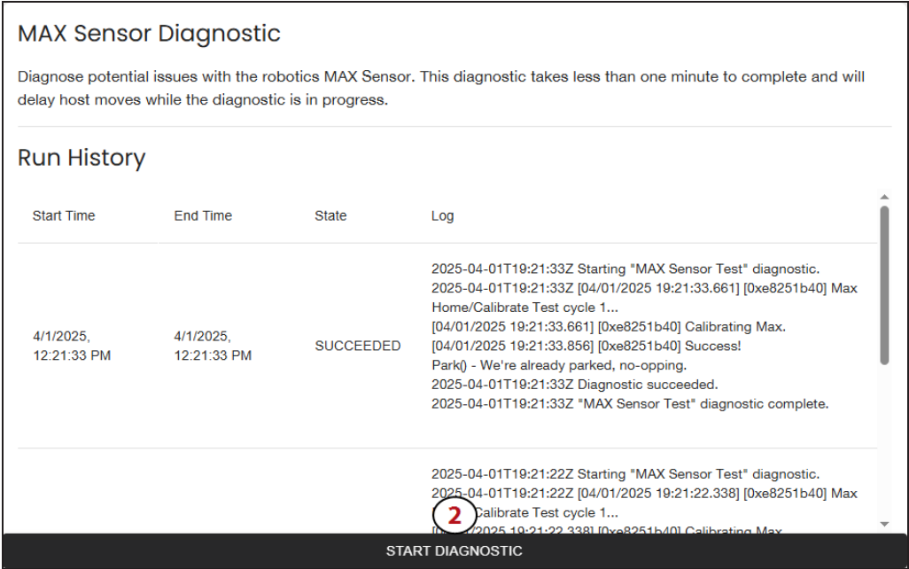
Figure 103 The LumOS MAX Sensor Diagnostic screen.
