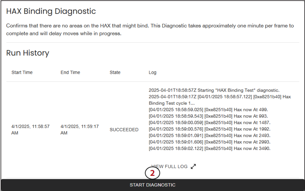
Figure 101 The LumOS HAX Binding Diagnostic screen.
