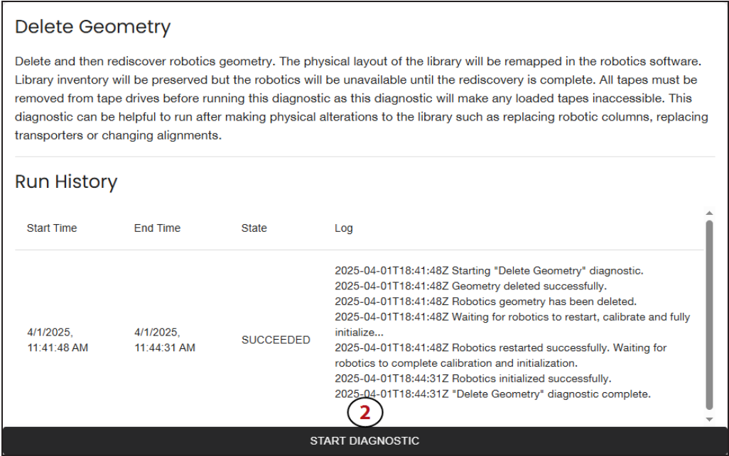
Figure 100 The LumOS Delete Geometry screen.
