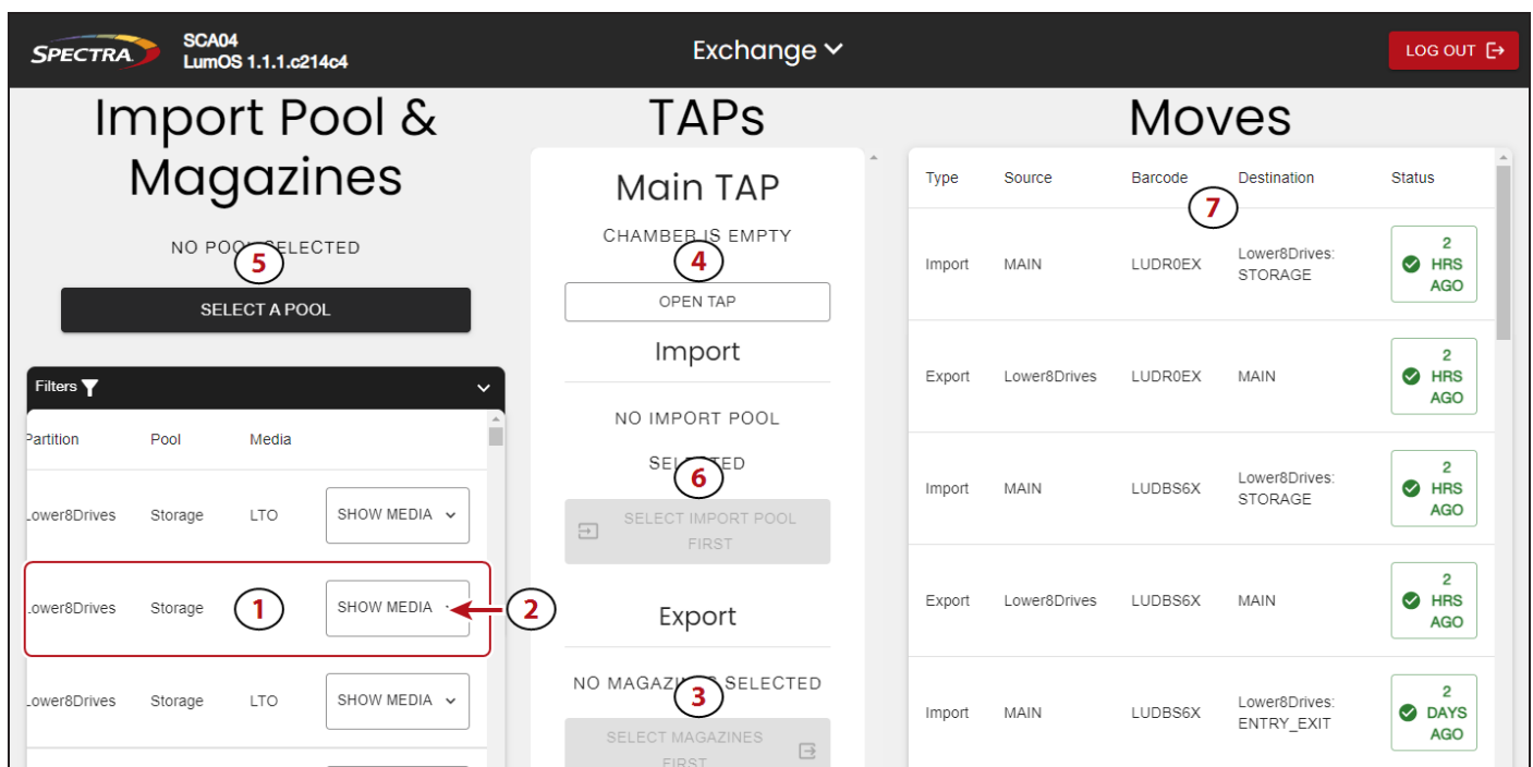
Figure 78 The LumOS Exchange screen.
