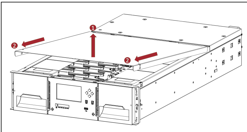
Figure 7 Remove the top cover from the base module.
