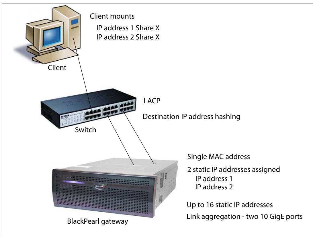
Figure 1 Connection example utilizing two IP addresses assigned to a single share.
